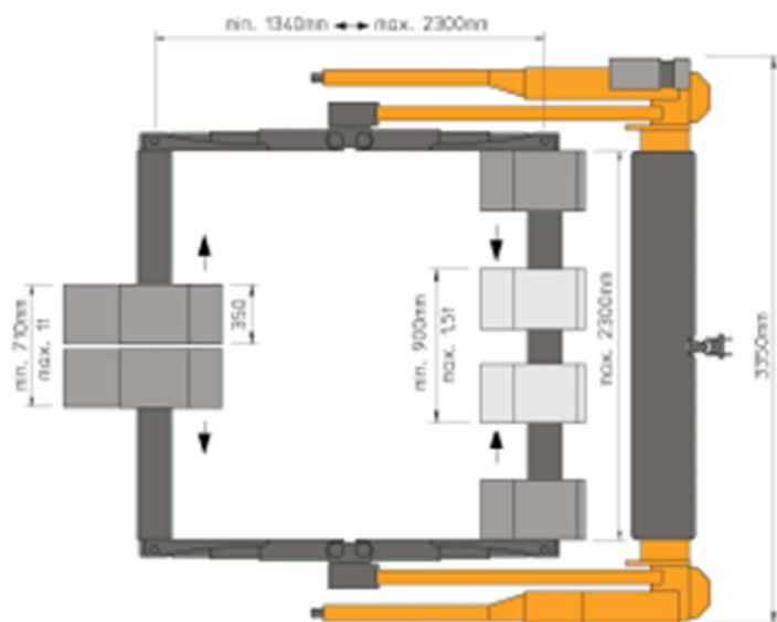
Pic. FHB3000-SS-2300 with ascending device FA-TORO
